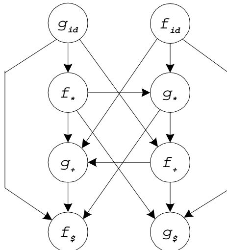
Figure 2: Graph representing precedence functions
