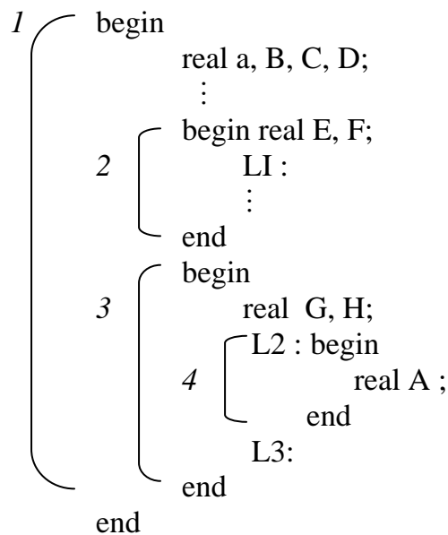
Figure 4: Block Structured Program
