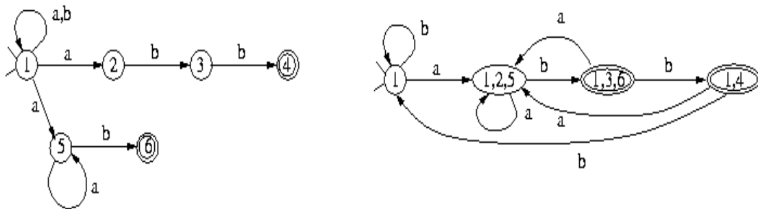
Figure 8: NFA recognising (a|b)^*(abb|a^+b)
