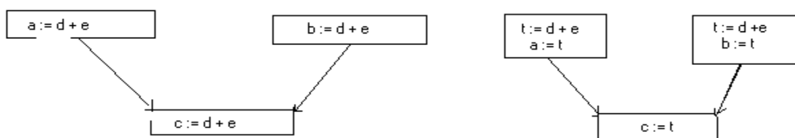
Figure 2: Copies introduced during common subexpression elimination.
