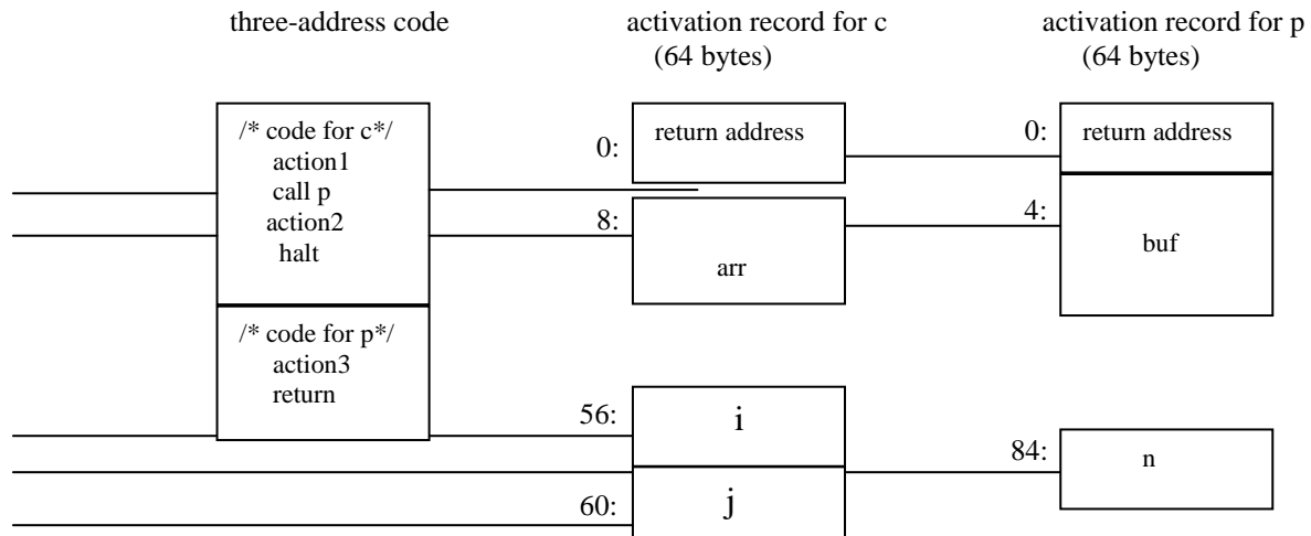
Figure 4: Input to a code generator
