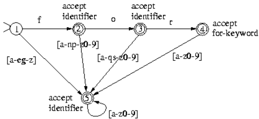
Figure 3: DFA recognising identifier and for-keyword
