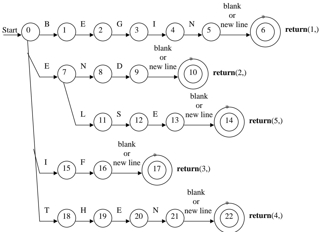
Figure 3: Transition diagram for keywords
