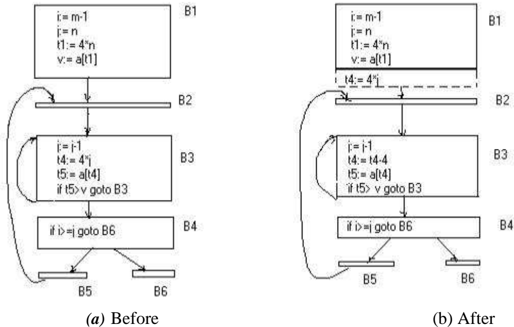
Figure 1: Strength reduction applied to 4*j in block B 3
