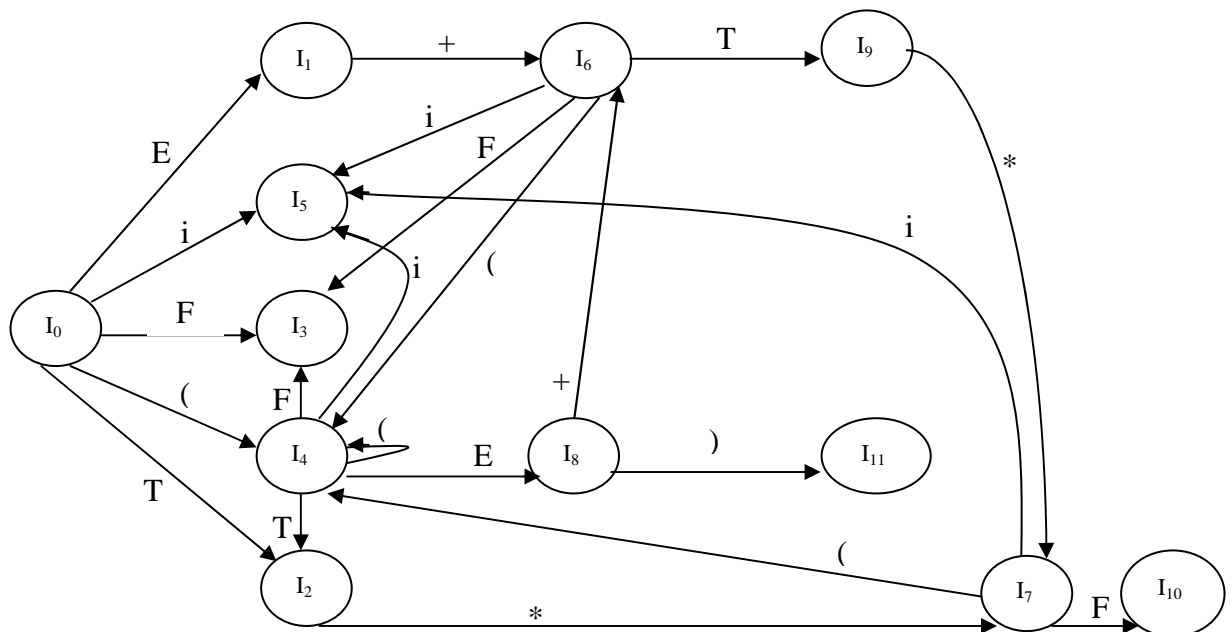
Figure 5: Deterministic Finite Automaton D
