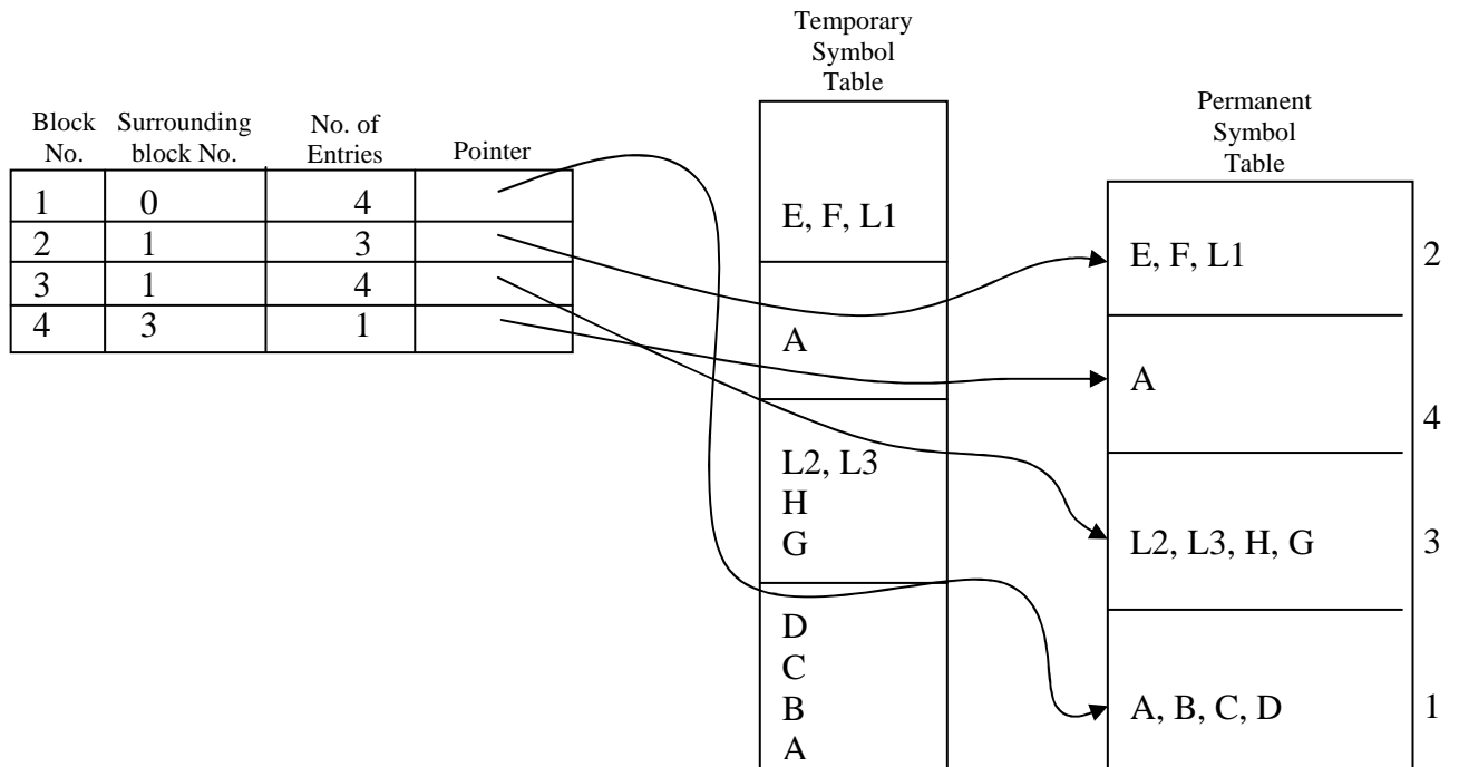
Figure 5: Symbol Table for the Block Structured Program
