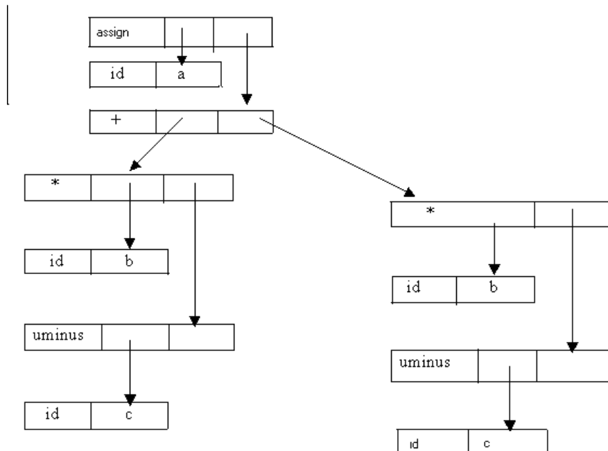
Figure 3(a): Two representations of the syntax tree
