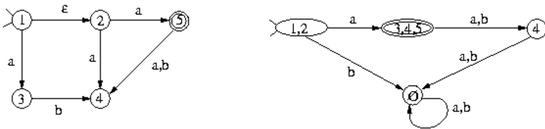
Figure 7: Closure of NFA
