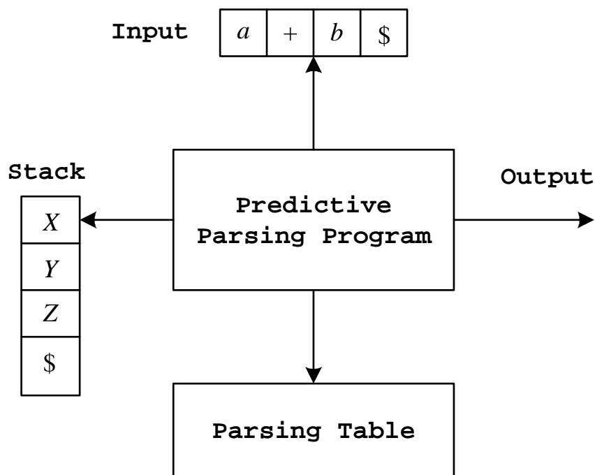
Figure 1: Model of a predictive parser
