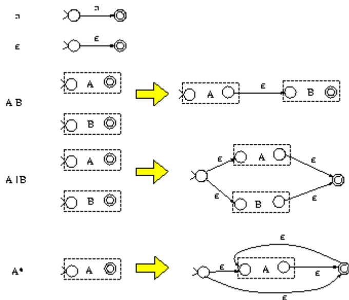
Figure 4: NFA for each RE characteristics
