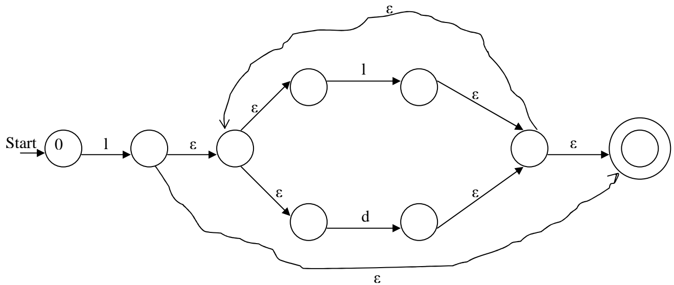
Figure 6: NFA recognising identifier
