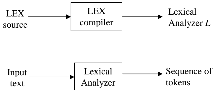
Figure 1: The role of LEX
