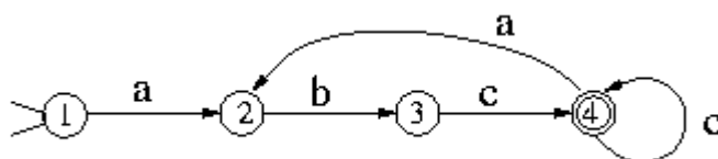
Figure 1: DFA recognising the string (abc^+)^+
