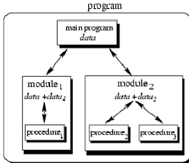
Figure 1.4.1: Modular Programming
