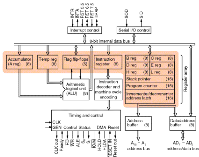
Figure 1: Architecture of 8085 Microprocessor
