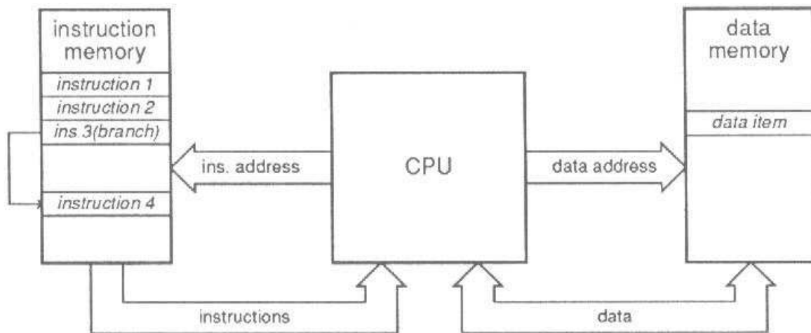
Figure 6 : Harvard Architecture
