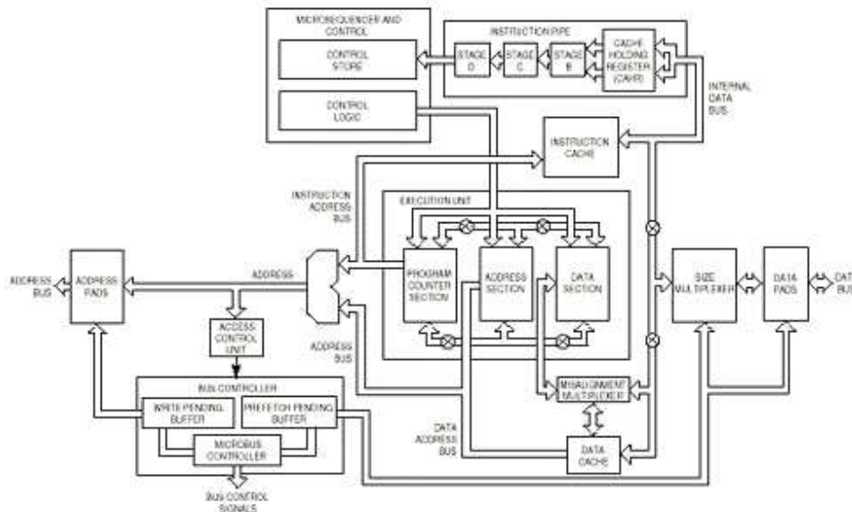
Figure 2: Motorola Microprocessor
